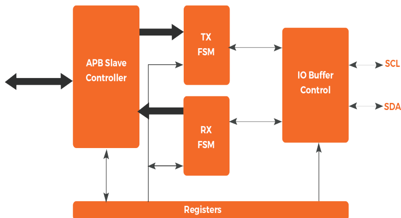
Block Diagram: I2C Controller
